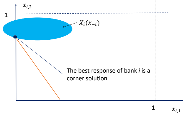
Figure 3: The point-to-set map of a given bank
