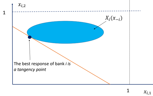
Figure 2: The point-to-set map of a given bank
