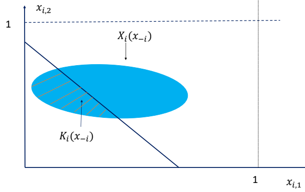
Figure 5: The point-to-set map K_i(x_{-i}) \subset X_i(x_{-i})
