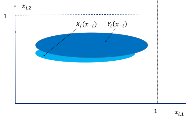
Figure 4: Risk-based capital ratio and leverage ratio
